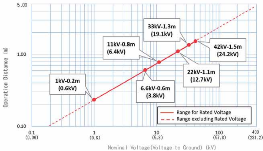
Operation Voltage Distance graph (Theoretical value)
