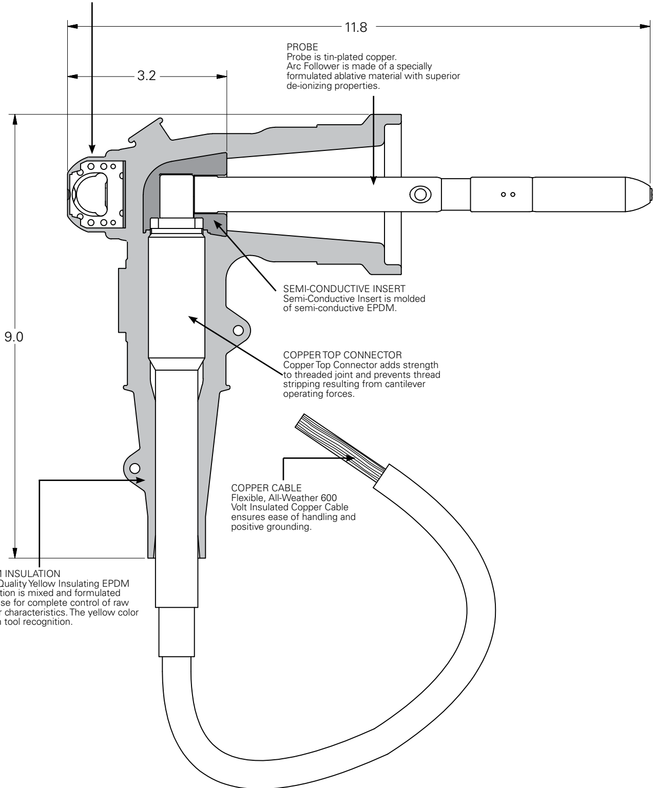
Figure 1. GE625 15 and 25 kV grounding elbow.
