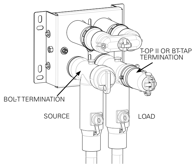
Figure 9. 600 A, 25 kV loadbreak connector system with (1) BOLT and (1) T-OP II or BT-TAP termination.
