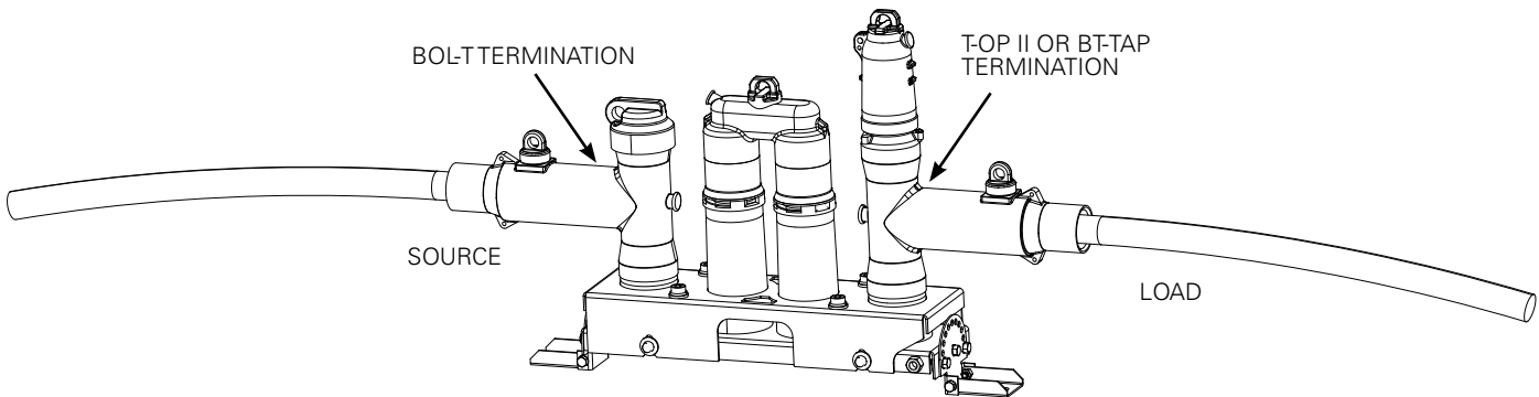
Figure 7. 600 A, 25 kV loadbreak connector system with (1) BOLT and (1) T-OP II or BT-TAP termination.
