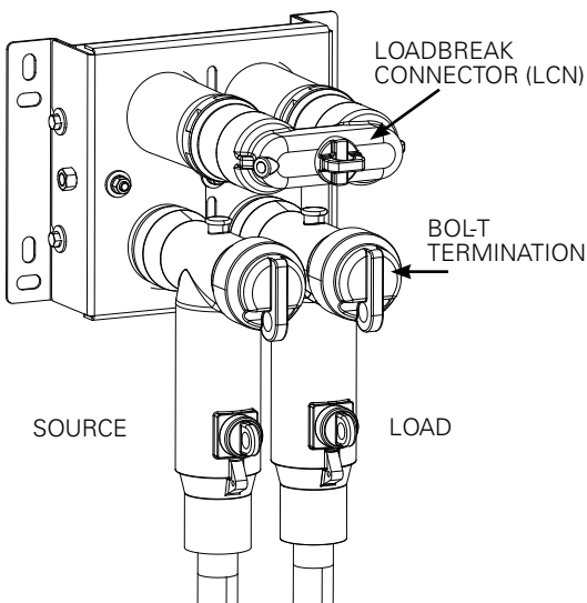
Figure 8. 600 A, 25 kV loadbreak connector system with (2) BOLT terminations.
