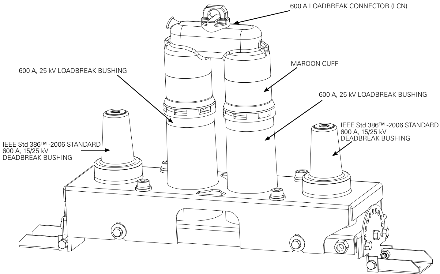
Figure 1. 600 A, 25 kV Cleer loadbreak connector system with in-line bracket.
