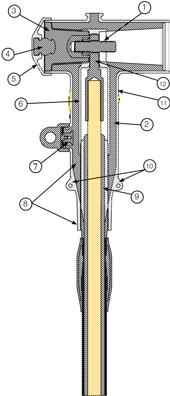
Figure 1. 630 A, 24 kV Class DTS624 deadbreak tee connector.
