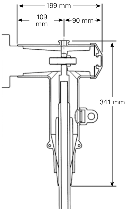
Figure 2. DTS624 deadbreak tee connector dimensional information.
