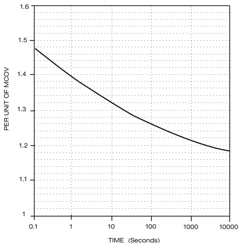
Figure 8. Temporary Overvoltage Capability.
