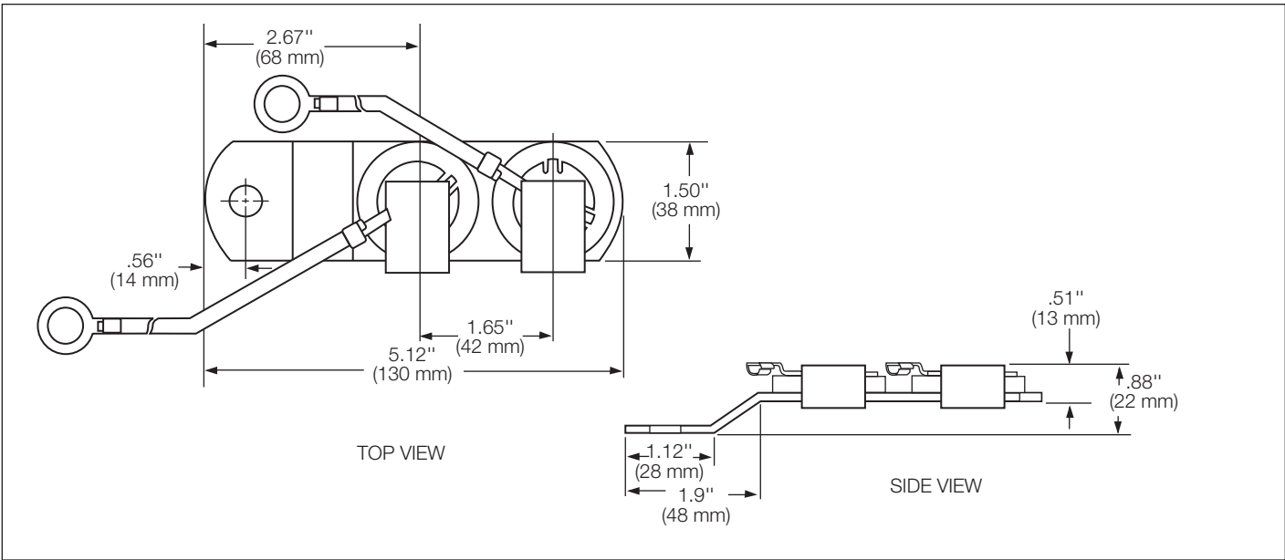
Figure 7. Dimensional information for internal mount Storm Trapper H.E. arrester (shown with optional terminal lugs).
