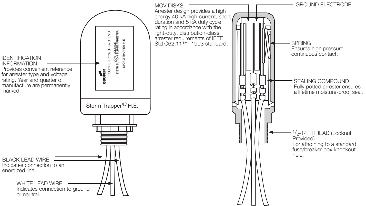
Figure 4. Cutaway Illustration of external mount Storm Trapper H.E. arrester without mounting bracket (two pole model illustrated).
