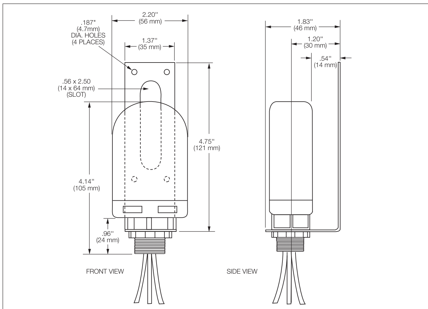
Figure 5. Dimensional information for external mount Storm Trapper H.E. arrester (shown with optional mounting bracket).
