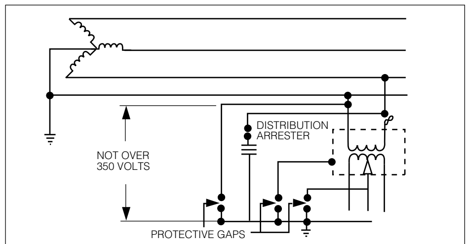
Figure 13. Typical application of protective gaps.
