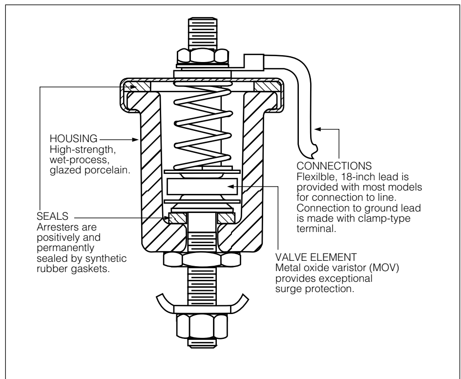
Figure 8. Cutaway illustration Type S4, 650 V secondary arrester.
