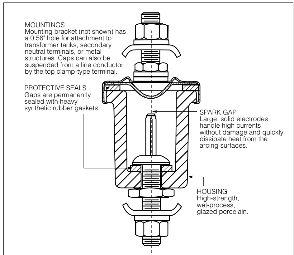
Figure 12. Cutaway illustration of protective gap.
