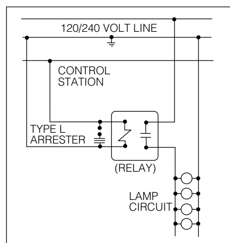
Figure 6. A typical multiple street lighting control circuit showing Type L secondary arresters protecting the relay coil.
