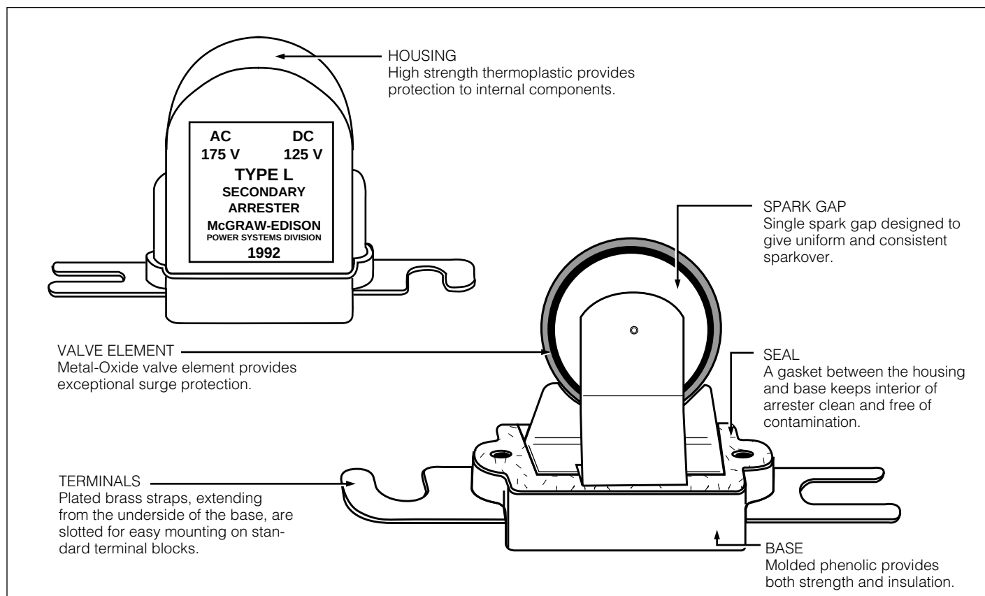
Figure 4. Cutaway illustration of Type L (175 Vac, 125 Vdc) secondary arrester.
