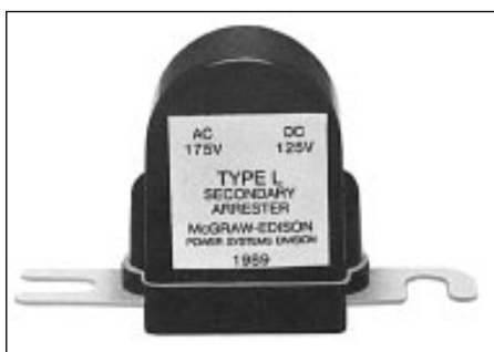
Figure 1. Type L secondary surge arrester—rated 175 Vac, 125 Vdc.
