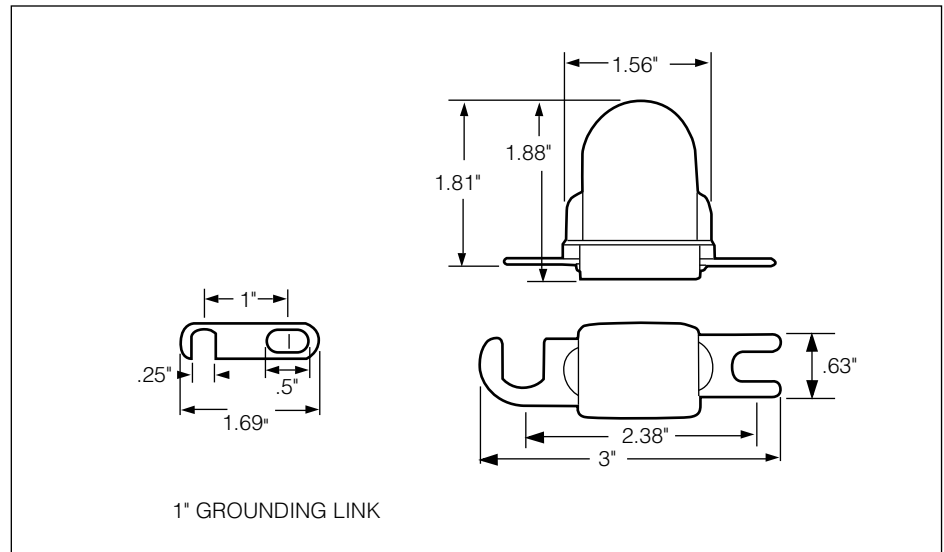
Figure 7. Type L secondary arrester dimensional information.
