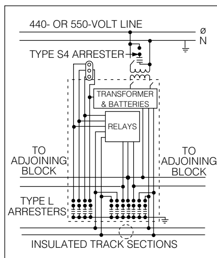
Figure 5. Railway application diagram showing an automatic railway block signal control with Cooper Power Systems Type L secondary arresters. One arrester is used on each outgoing line.
