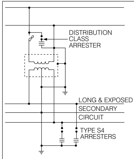
Figure 9. Typical application of Type S4 arresters protecting long and exposed secondary lines in oil field or rural areas.
