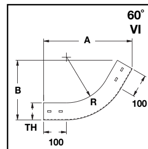
60° Vertical Inside
