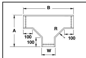
Horizontal Tee Mitered (R) Shown
