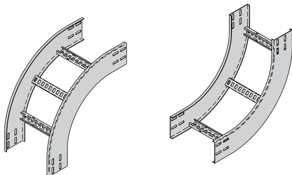
90° Vertical Outside
