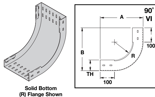
90° Vertical Inside
