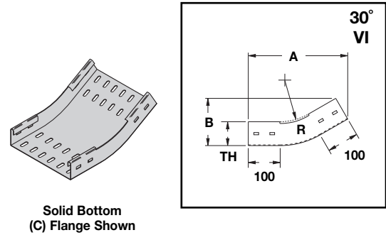
30° Vertical Inside
