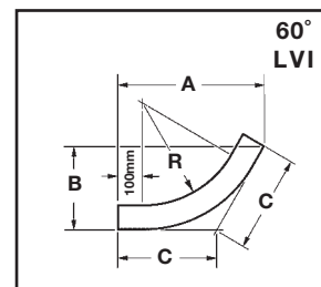
60° Vertical Inside
