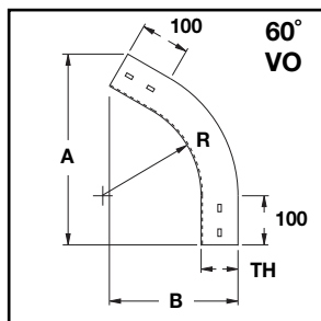
60° Vertical Outside
